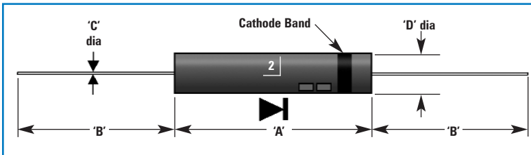
Dimension Details
