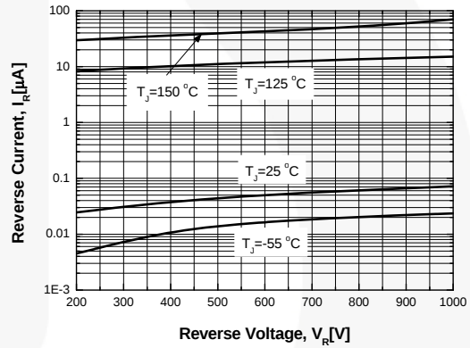
Figure 6. Reverse Current vs. Reverse Voltage
