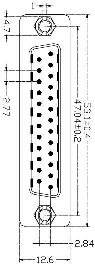
DB25M
