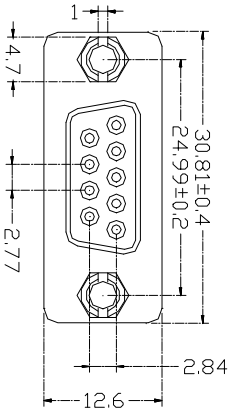
DB9F
