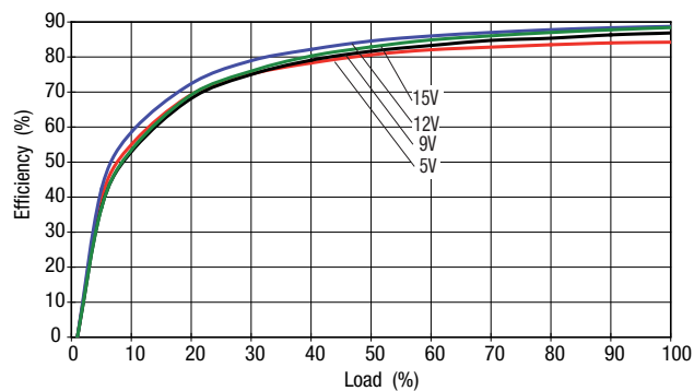
MEV1x24xxSC
