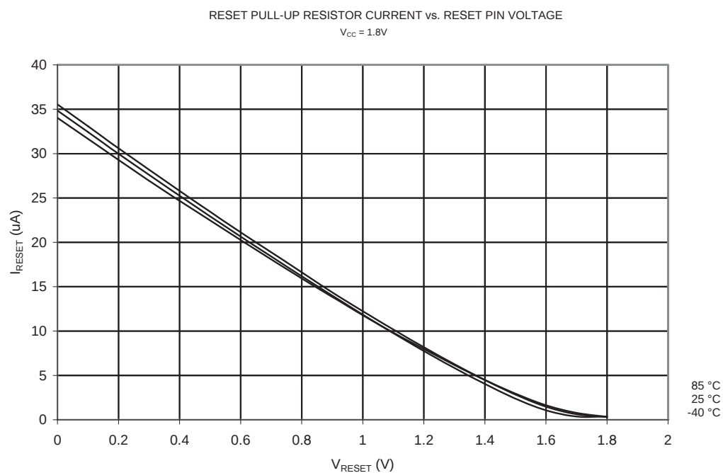
Figure 20-23. Pull-Up Resistor Current vs. Input Voltage (Reset Pin, V_{CC} = 1.8V )
