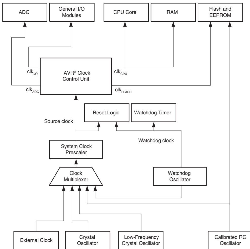
Figure 6-1. Clock Distribution
