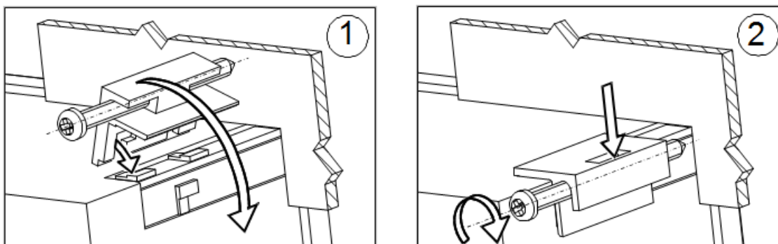
Fig.2. Meter fixing
