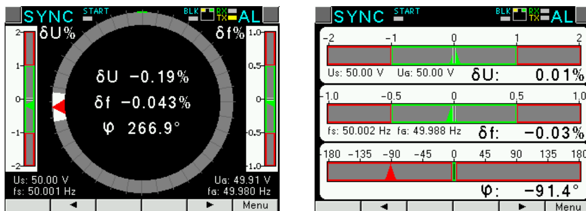
Fig.9, Visualization of measurements (synchronoscope, bar graphs)*
