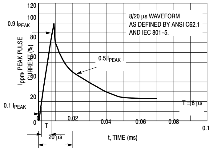
Figure 10. Pulse Waveform
