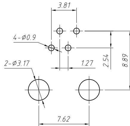
PCB Layout
