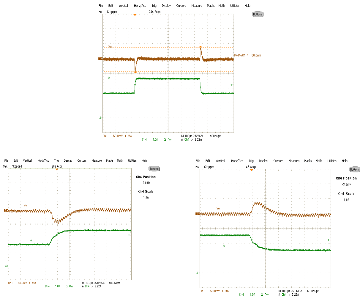
Fig. 23. Transient Response, 1A to 2A step 2.5\text{A}/\mu\text{s} \text{Ch}_1:\text{V}_o, \text{Ch}_4:\text{I}_o
