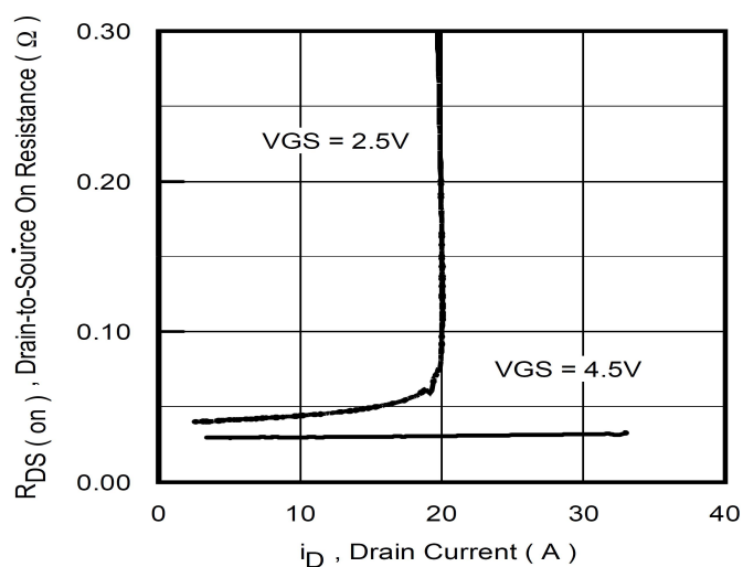
Fig 12. On-Resistance Vs. Drain Current
