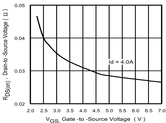
Fig 11. On-Resistance Vs. Gate Voltage
