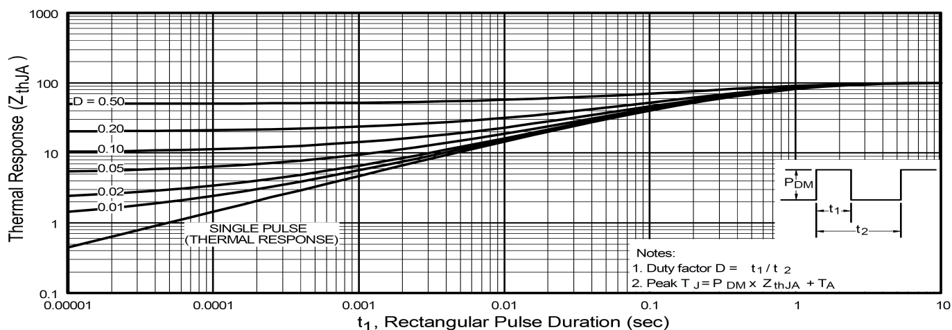
Fig 10. Maximum Effective Transient Thermal Impedance, Junction-to-Ambient
