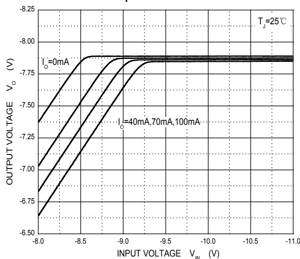
Dropout Characteristics
