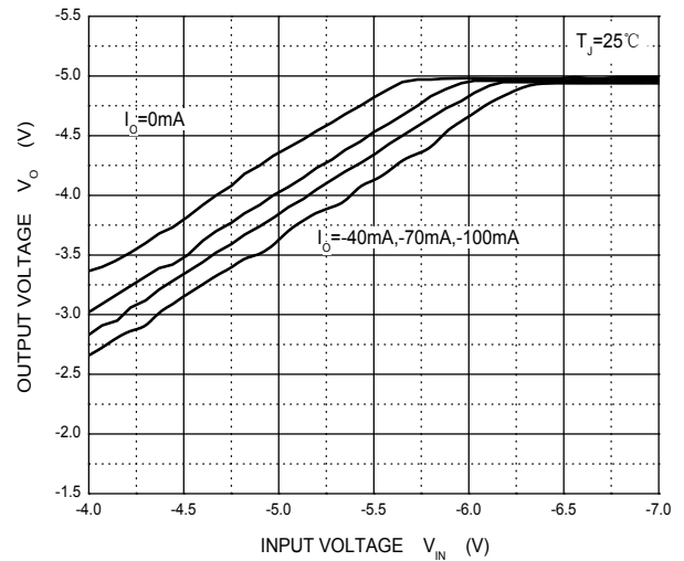
Dropout Characteristics
