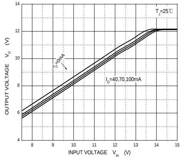
Dropout Characteristics
