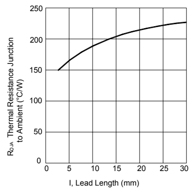
Fig. 2 Typical Thermal Resistance vs. Lead Length
