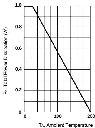
Fig. 1 Power Dissipation vs. Ambient Temperature
