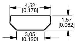
Figure 3. Mounting Dimensions (For reference only. mm/in.)
