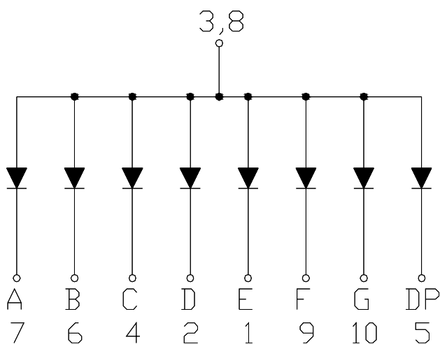
Common Anode
