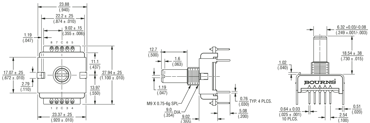
PCB Bracket Mounted: Housing B
