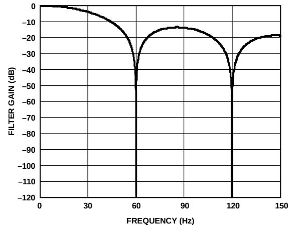
Figure 111. 60 Hz Rejection
