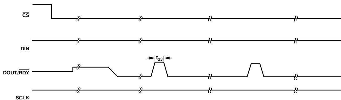
Figure 7. DOUT/\overline{RDY} High Time when DOUT/\overline{RDY} is Initially Low and the Next Conversion is Available
