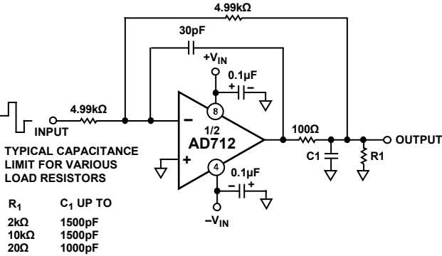
Figure 46. Circuit for Driving a Large Capacitive Load
