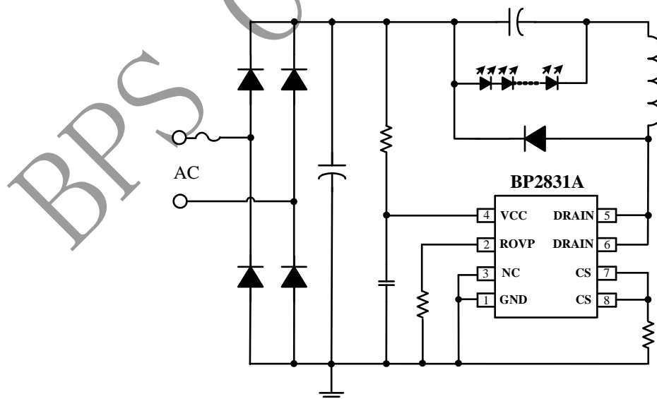
Figure 1. Typical application circuit for BP2831A
