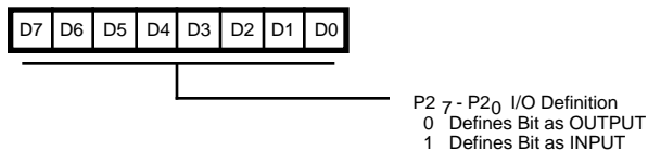
Figure 21. Port 2 Mode Register (F6 H : Write Only)
