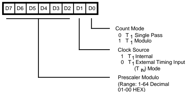
Figure 20. Prescaler1 Register (F3 H : Write Only)
