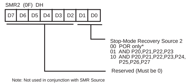
Figure 38. Stop-Mode Recovery Register2
