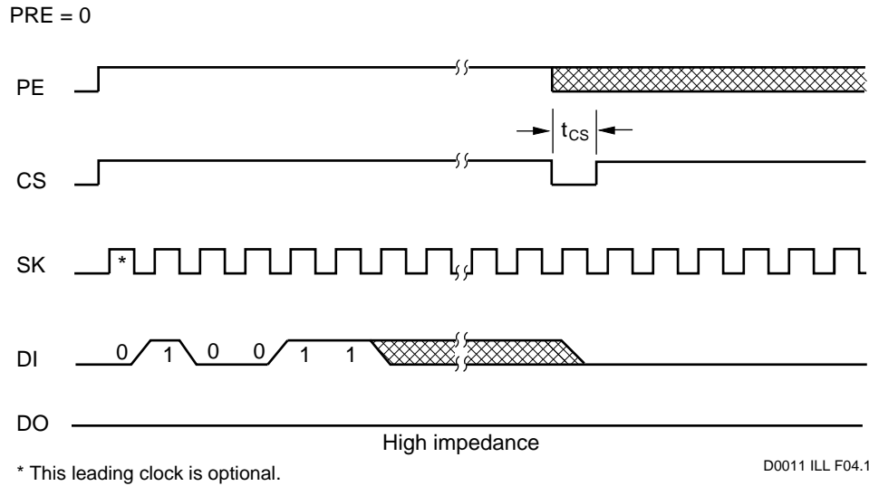
FIGURE 4. WRITE ENABLE (WEN) CYCLE TIMING
