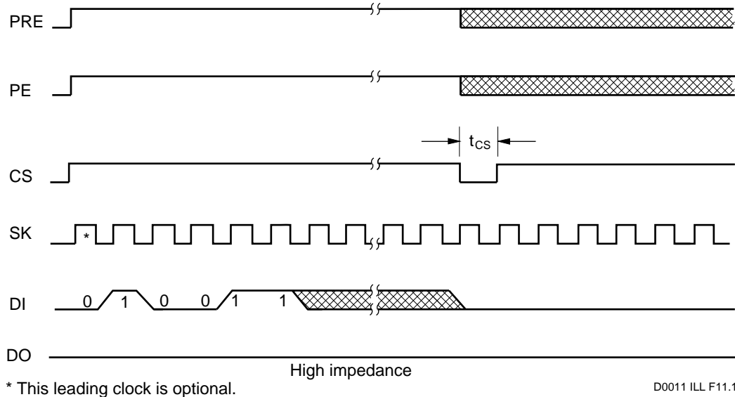
FIGURE 11. PROTECT REGISTER ENABLE (PREN) CYCLE TIMING
