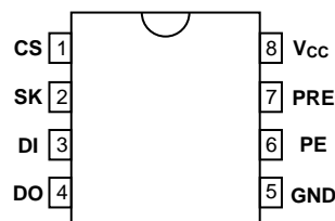
Plastic Dual-in-line Type "P" Package
