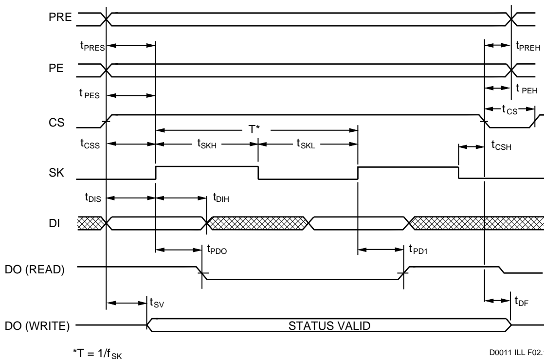
FIGURE 2. SYNCHRONOUS DATA TIMING
