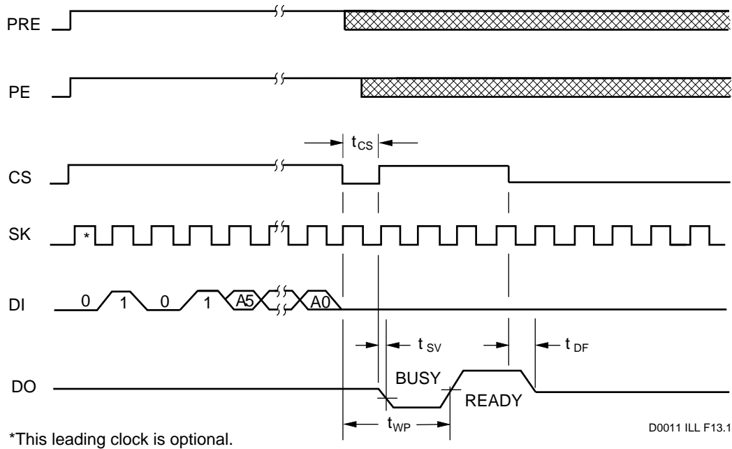
FIGURE 13. PROTECT REGISTER WRITE (PRWRITE) CYCLE TIMING
