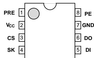
EIAJ Small Outline "J" Package
