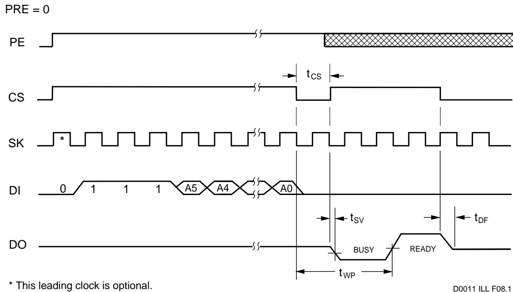
FIGURE 8. ERASE (REGISTER) CYCLE TIMING
