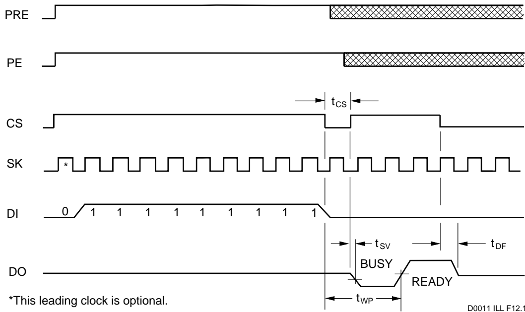
FIGURE 12. PROTECT REGISTER CLEAR (PRCLEAR) CYCLE TIMING
