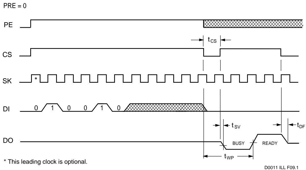
FIGURE 9. ERASE ALL (ERAL) CYCLE TIMING
