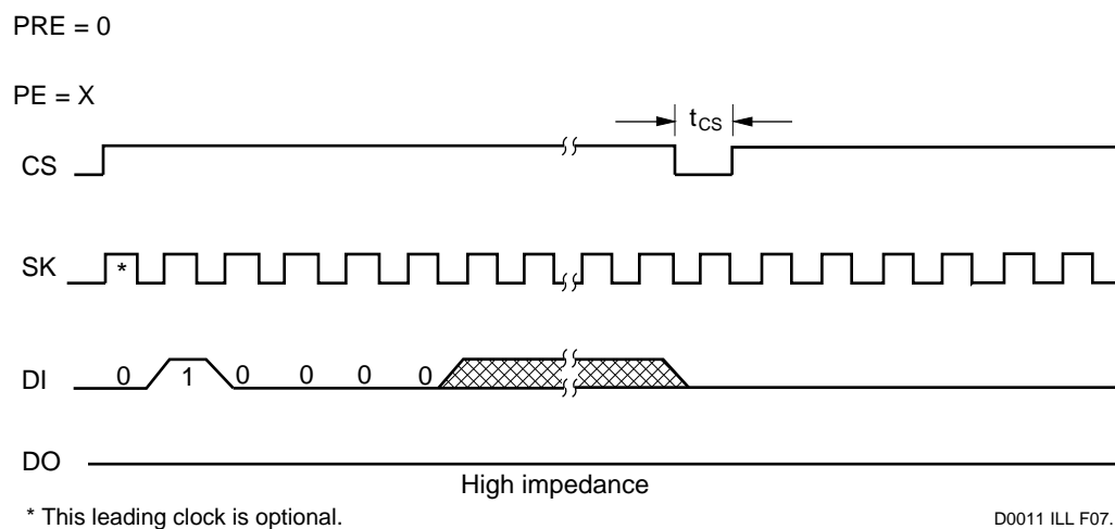
FIGURE 7. WRITE DISABLE (WDS) CYCLE TIMING
