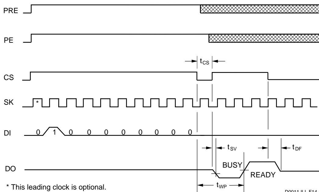
FIGURE 14. PROTECT REGISTER DISABLE (PRDS) CYCLE TIMING
