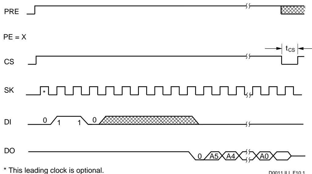
FIGURE 10. PROTECT REGISTER READ (PREAD) CYCLE TIMING
