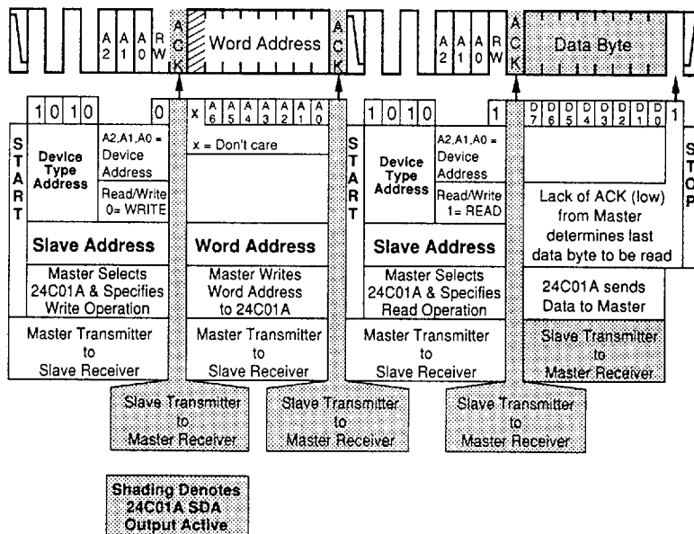
FIGURE 9. RANDOM ACCESS BYTE READ MODE
