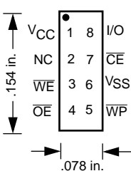
8-LEAD XBGA: Top View
