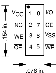
8-LEAD XBGA: Top View
