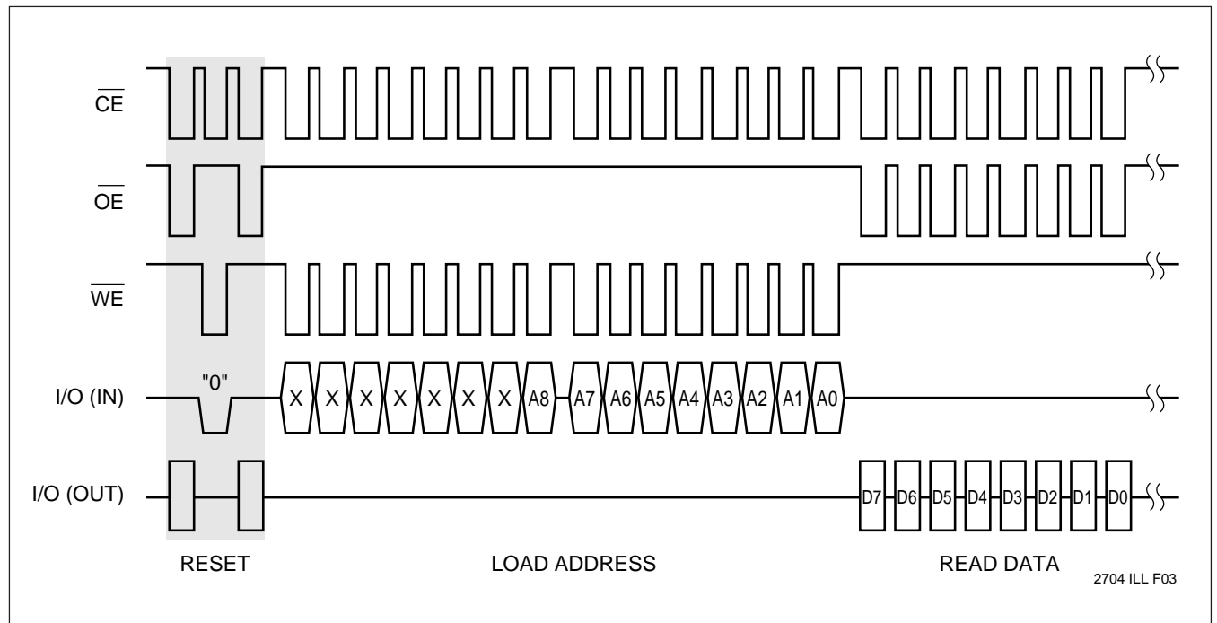
Figure 1. Read Sequence
