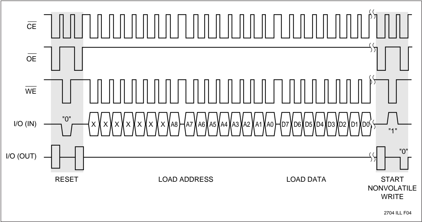
Figure 2. Write Sequence
