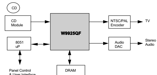
Figure 1.2 Application Example of W9925QF in Video CD Players
