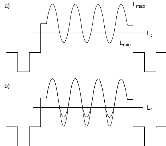
Fig. 2-12: Black-level expansion a) luminance input b) luminance input and output
