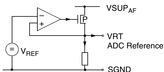
Fig. 6-13: Supply pins VRT, SGND
