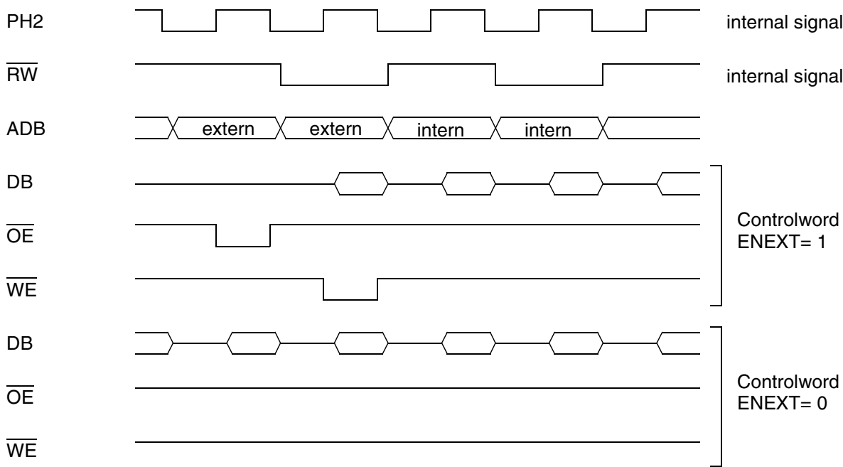
Fig. 5–2: Internal/external memory access
