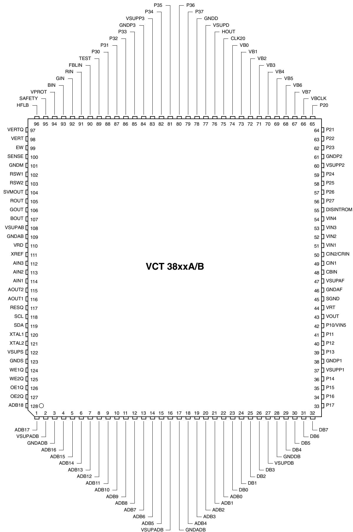
Fig. 6-4: PMQFP128 package
