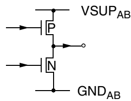
Fig. 6–19: Output pin INTLC
