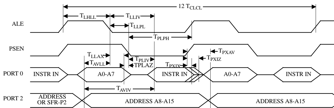
Figure 17. External Program Memory Read Cycle
