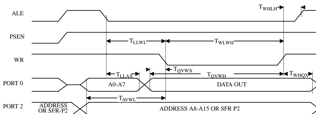
Figure 18. External Data Memory Write Cycle
