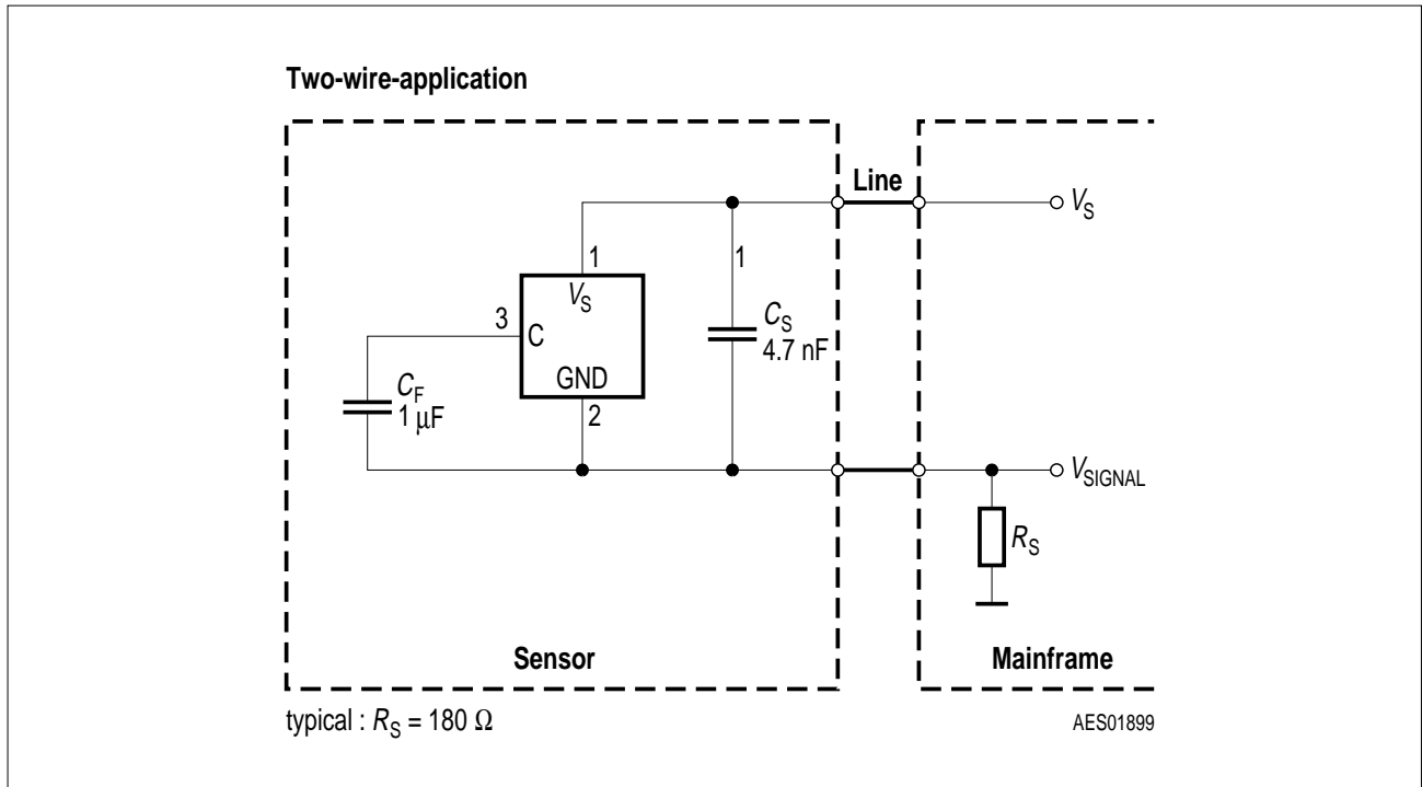
Figure 12 Application Circuit
