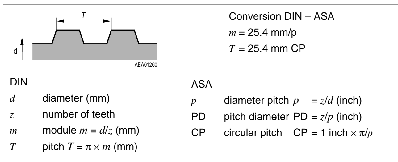
Figure 9 Tooth Wheel Dimensions
