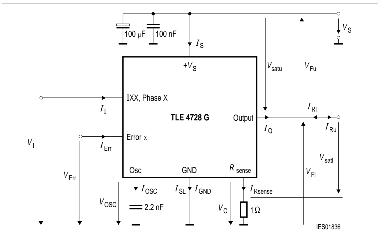
Figure 11 Test Circuit
