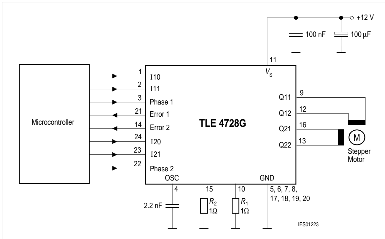
Figure 10 Application Circuit
