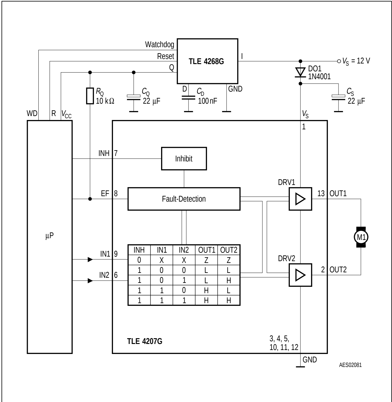
Figure 3 Application Circuit
