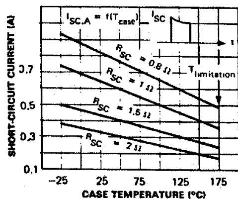
Short-circuit current versus case temperature
