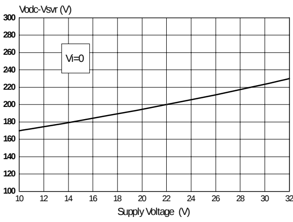
Output DC Offset vs. Supply Voltage
