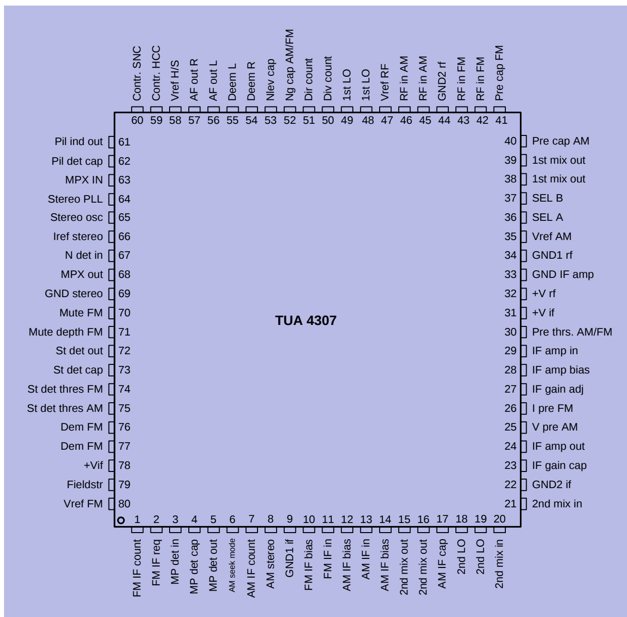
Figure 3-1 Pin Configuration
