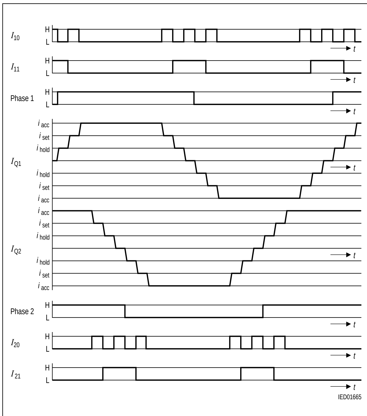
Figure 9 Mini-Step Operation
