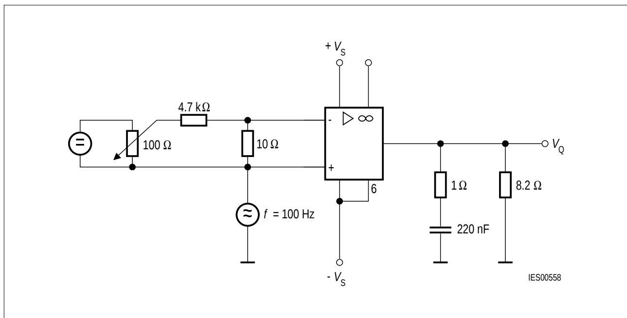
Figure 20 Common Mode Voltage Gain G_{VC} Common-Mode Rejection k_{CMR} \text{ (dB)} = G_{VO} \text{ (dB)} - G_{VC} \text{ (dB)} (TCA 2465/A)
