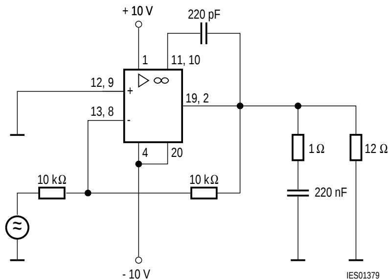
Figure 14 Inverting Operation (TCA 2465 G)
