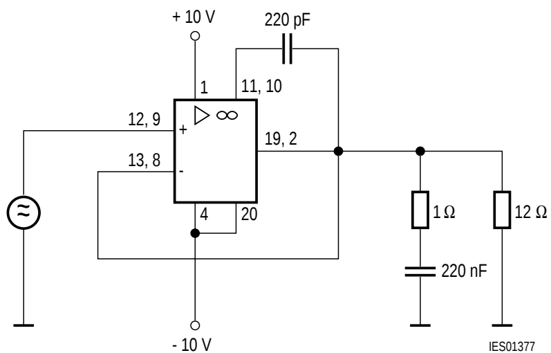
Figure 13 Non-Inverting Operation (TCA 2465 G)
