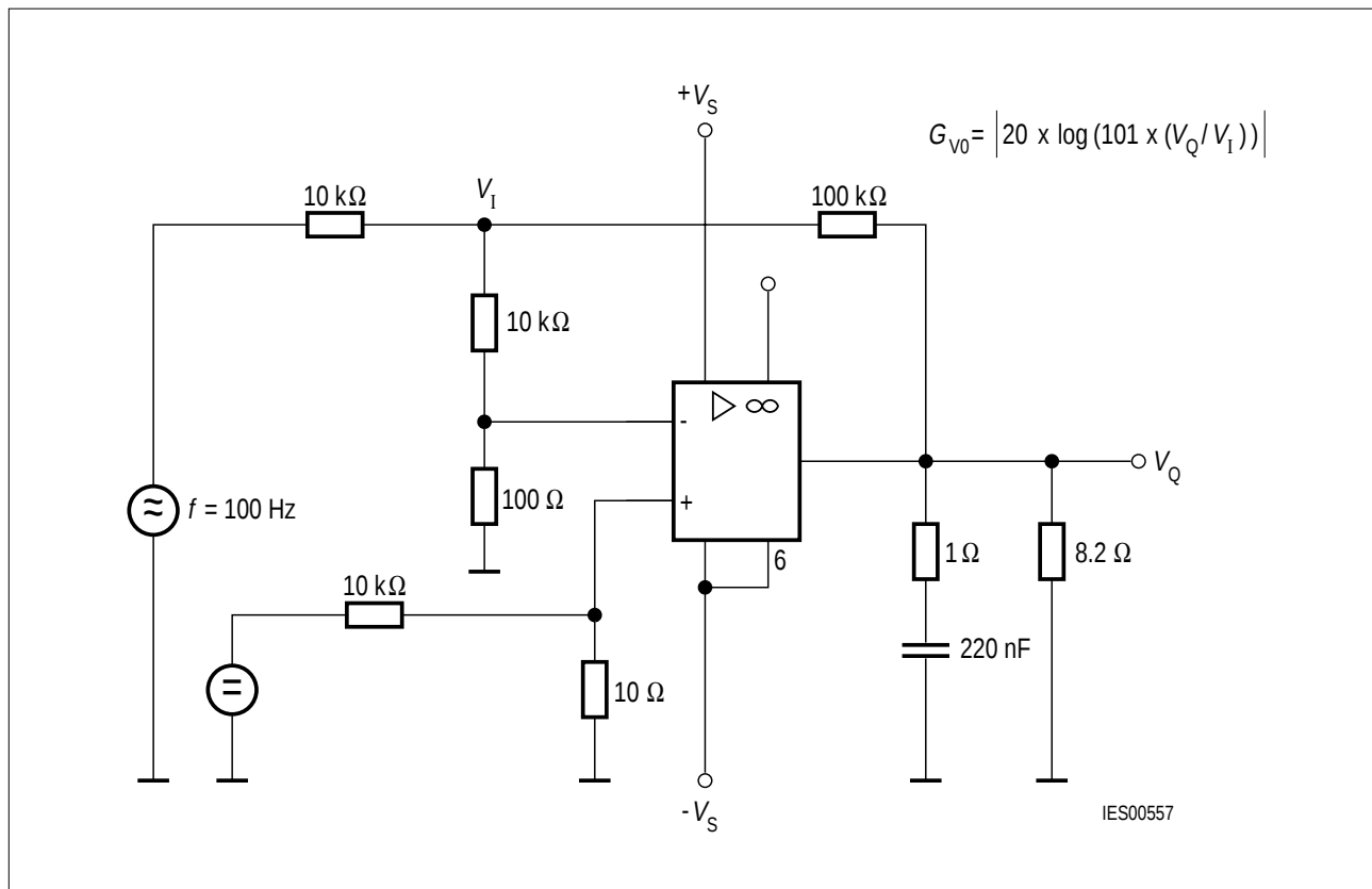
Figure 19 Open-Loop Voltage Gain G_{VO} (TCA 2465)
