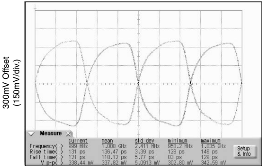
1GHz Output
