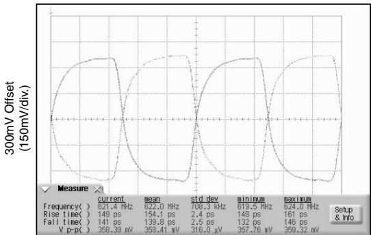
622MHz Output
