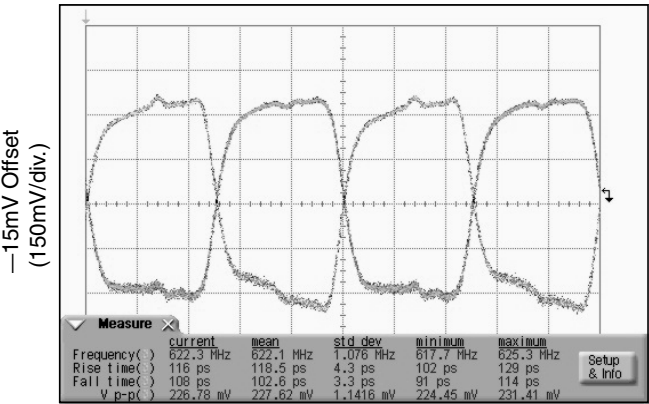
622MHz Output
