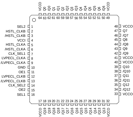
64-Pin TQFP (H64-1)
