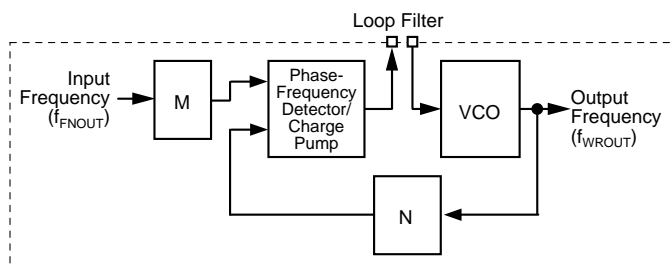
Figure 3. Wrapper Architecture
