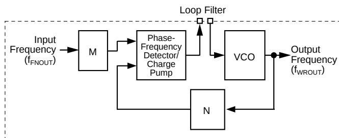
Figure 3. Wrapper Architecture
