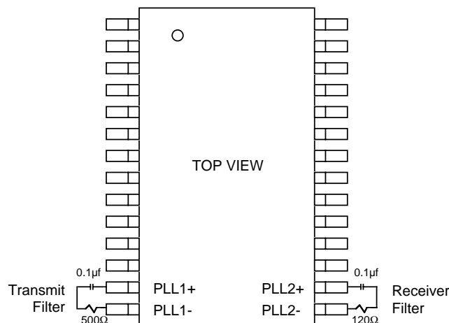
Figure 1. Suggested Loop Filter Values
