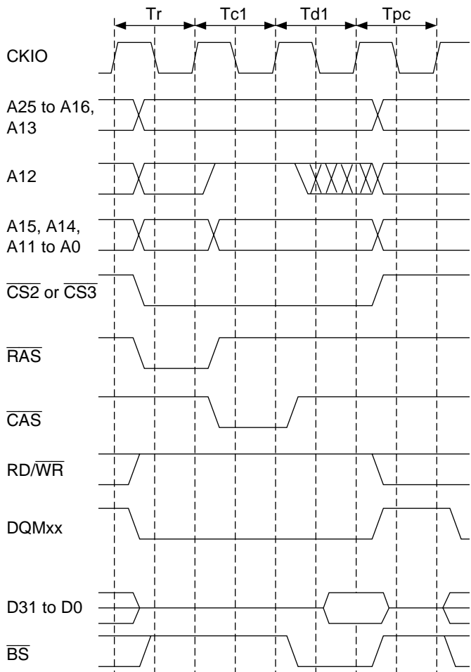
Figure 11.26 Basic Timing for Synchronous DRAM Single Read
