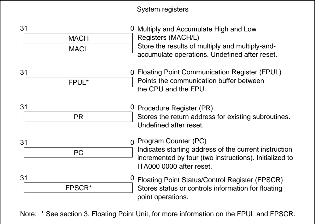
Figure 2.3 System Register Configuration
