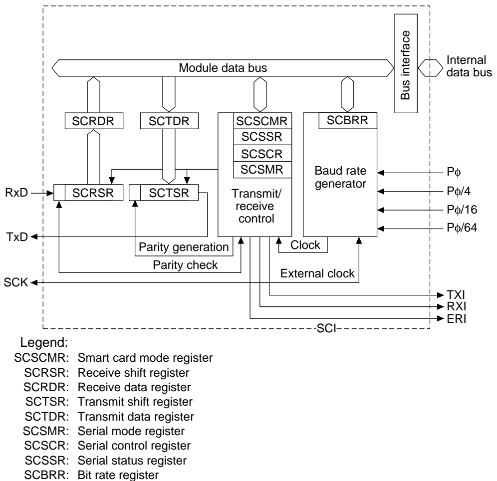
Figure 15.1 Smart Card Interface Block Diagram
