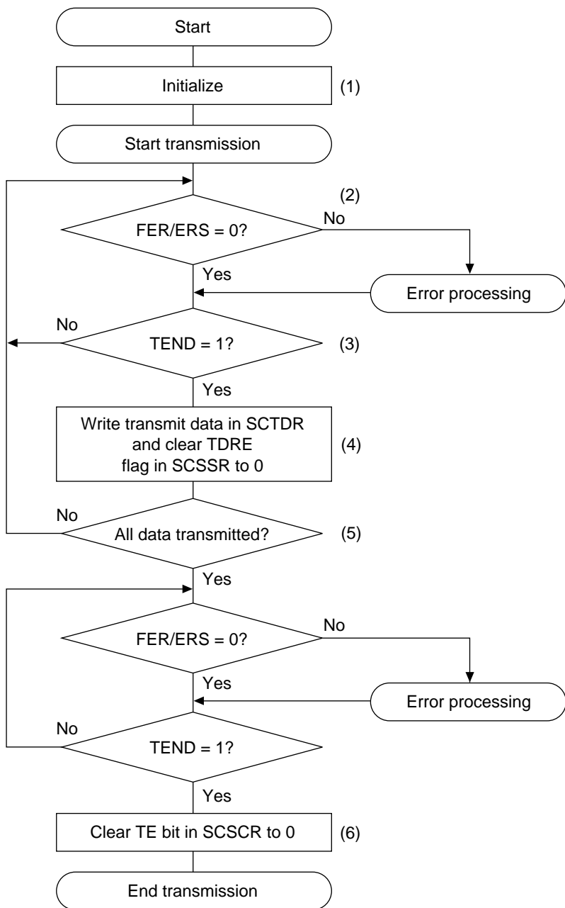
Figure 15.6 Transmission Flowchart
