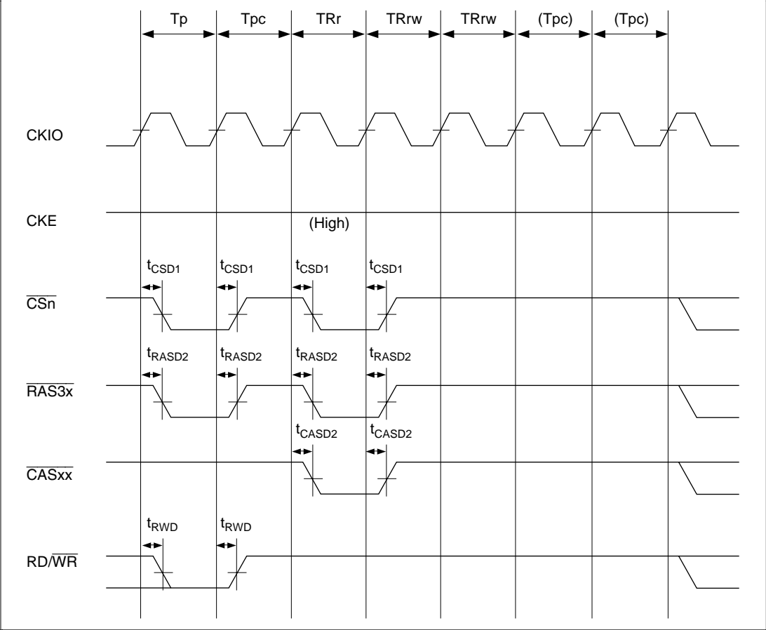
Figure 23.50 Synchronous DRAM Auto-Refresh Timing (TRAS = 1, TPC = 1)
