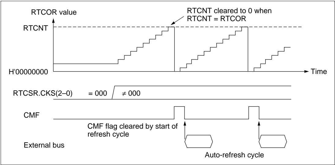
Figure 10.38 Auto-Refresh Operation
