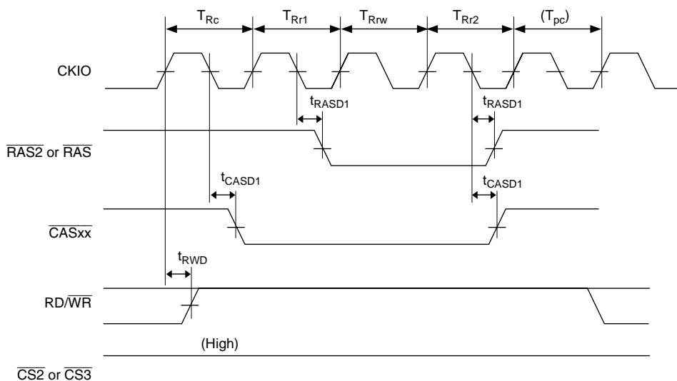
Figure 23.32 DRAM CAS-before-RAS Refresh Cycle (TRAS = 0, TPC = 0)
