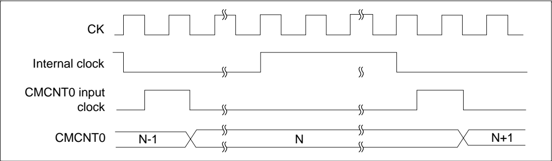
Figure 11.28 Count Timing
