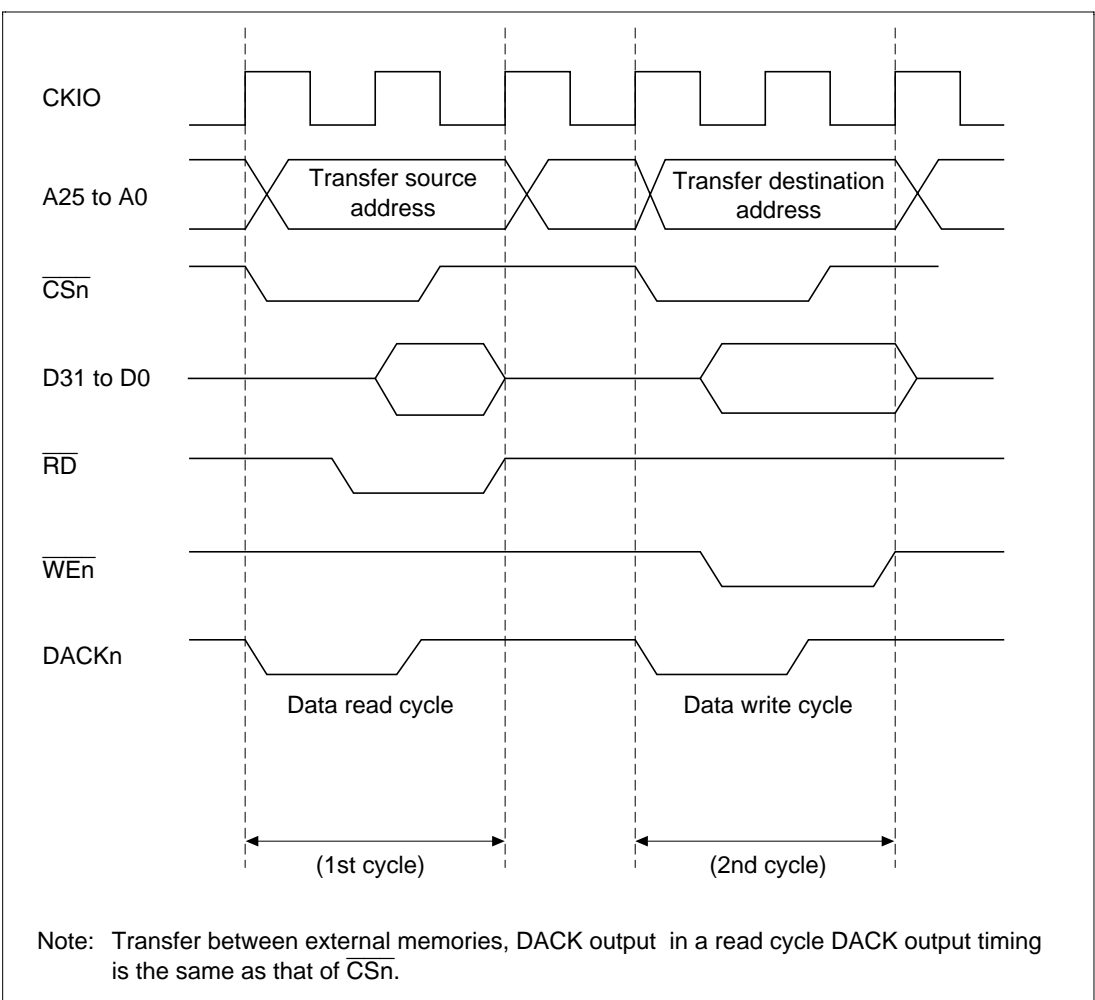
Figure 11.6 Example of DMA Transfer Timing in the Direct Address Mode in the Dual Mode
