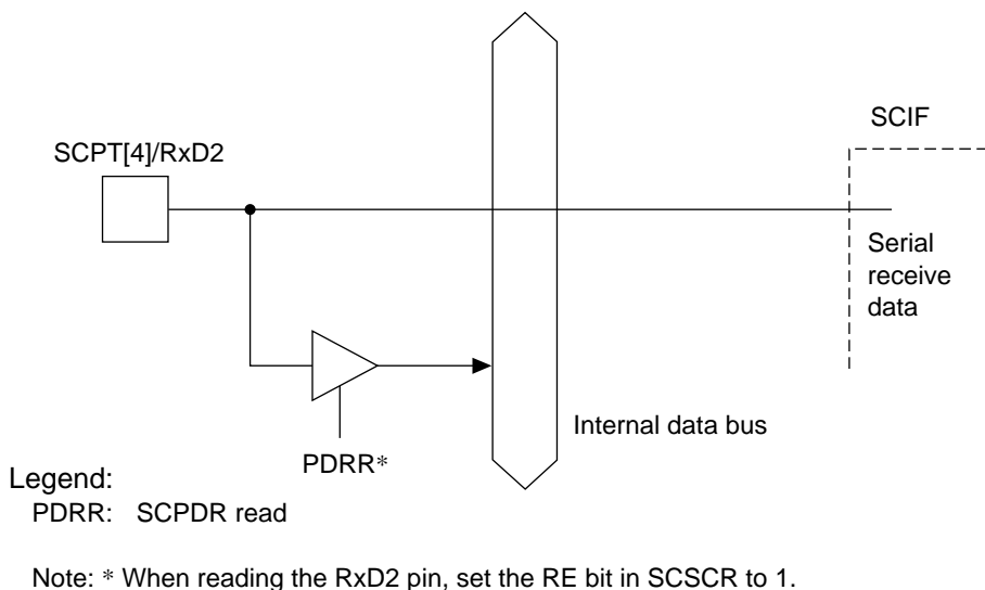
Figure 16.4 SCPT[4]/RxD2 Pin
