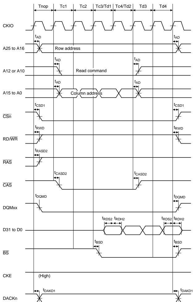
Figure 23.44 Synchronous DRAM Burst Read Bus Cycle (RAS Down, Same Row Address, CAS Latency = 2)
