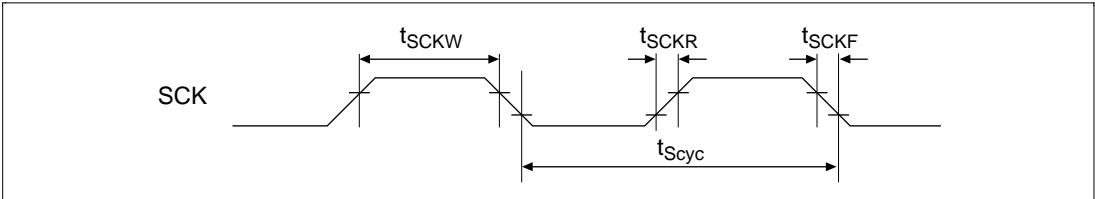
Figure 23.63 SCK Input Clock Timing
