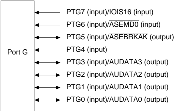
Figure 19.7 Port G
