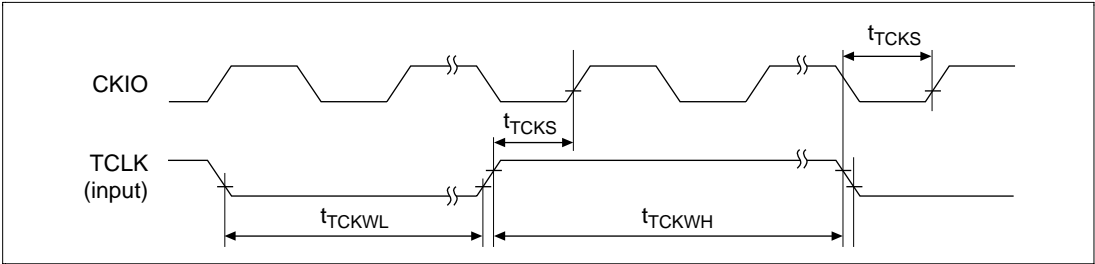
Figure 23.61 TCLK Clock Input Timing
