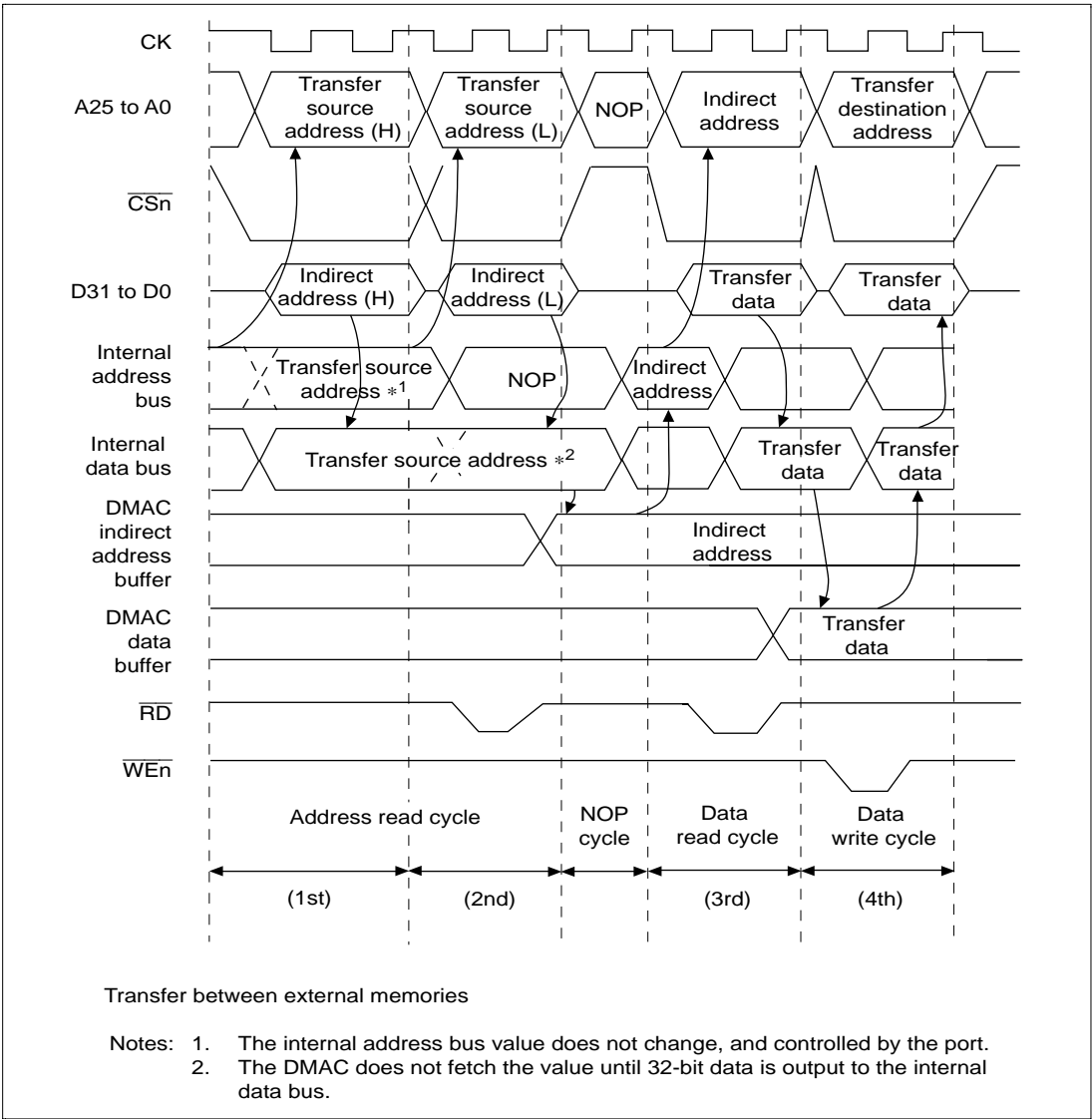
Figure 11.10 Example of Transfer Timing in the Indirect Address Mode in the Dual Address Mode
