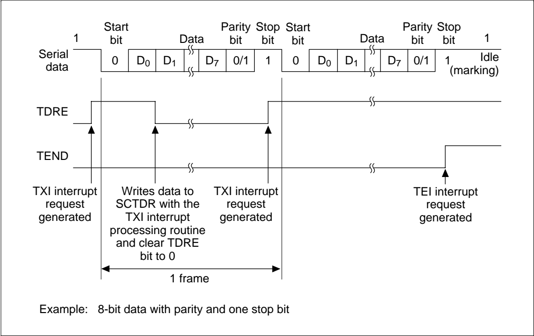
Figure 14.9 SCI Transmit Operation in Asynchronous Mode
