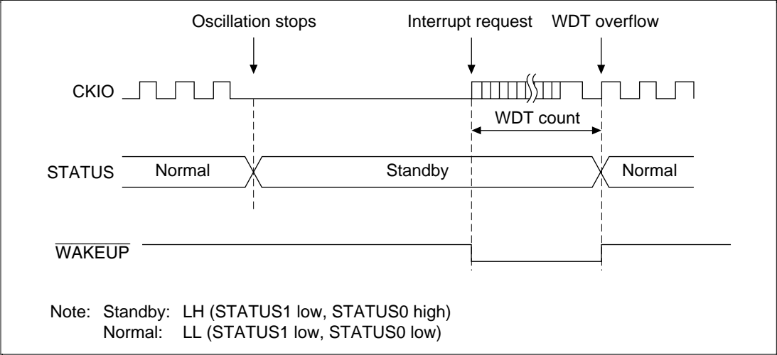
Figure 8.5 Standby to Interrupt STATUS Output
