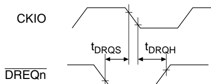
Figure 23.66 \overline{\text{DREQn}} Input Timing
