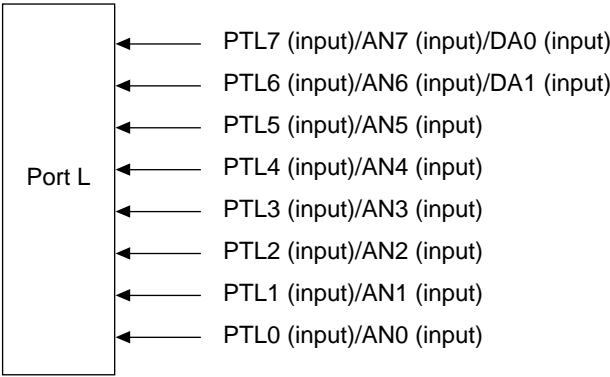
Figure 19.11 Port L
