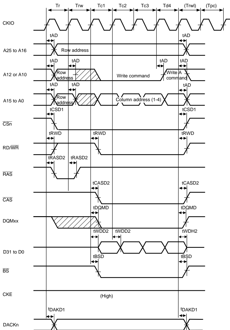
Figure 23.42 Synchronous DRAM Write Bus Cycle (Burst Mode (Single Write x 4), RCD = 1, TPC = 0, TRWL = 0)
