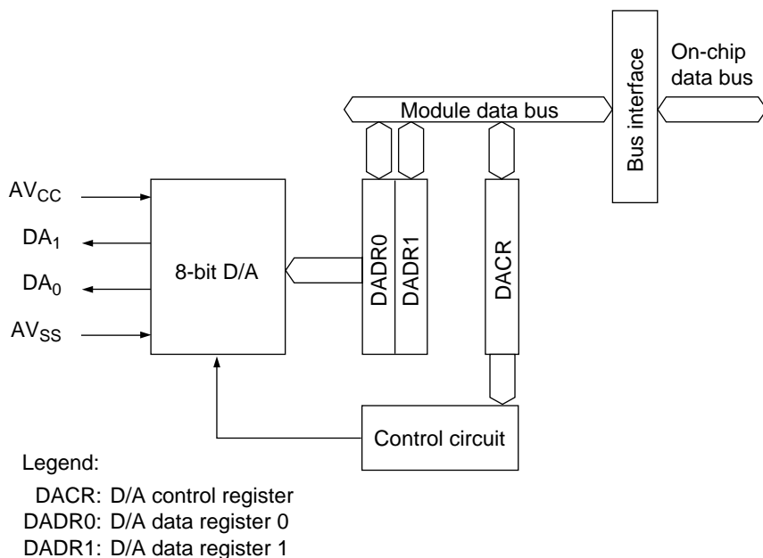
Figure 21.1 D/A Converter Block Diagram
