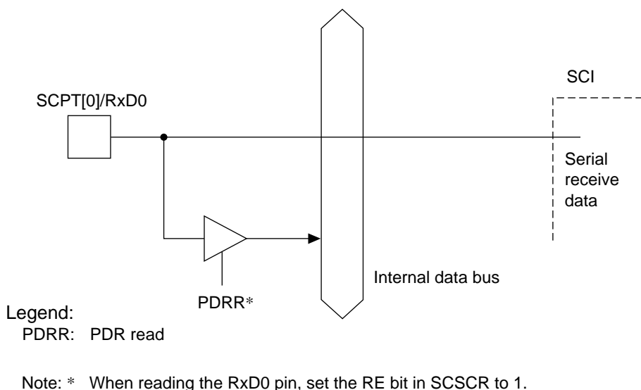
Figure 14.4 SCPT[0]/RxD0 Pin
