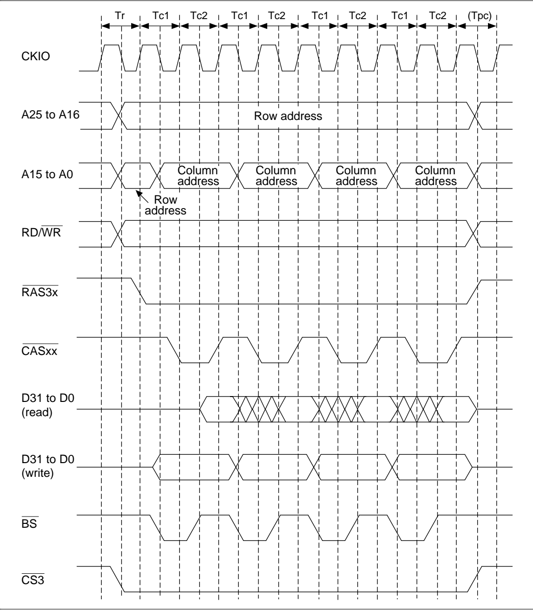
Figure 10.21 Burst Access Timing in DRAM EDO Mode
