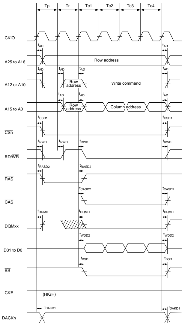
Figure 23.48 Synchronous DRAM Burst Write Bus Cycle (RAS Down, Different Row Address, TPC = 0, RCD = 0)
