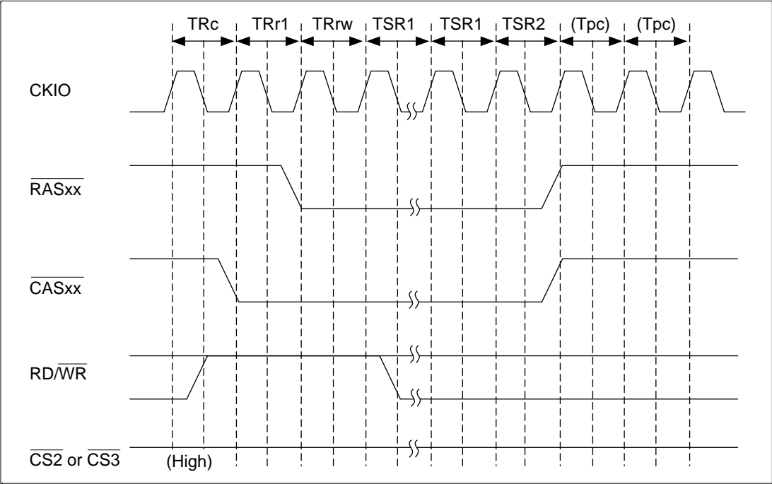
Figure 10.24 DRAM Self-Refresh Cycle Timing
