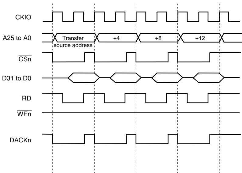
Figure 11.13 Example of DMA Transfer Timing in Single Address Mode (External Memory Space (Ordinary Memory) -> External Device with DACK)
