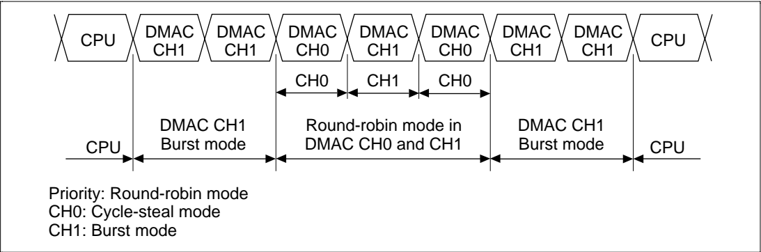
Figure 11.16 Bus State when Multiple Channels Are Operating
