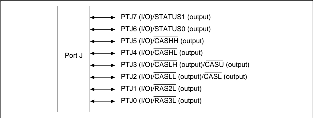
Figure 19.9 Port J
