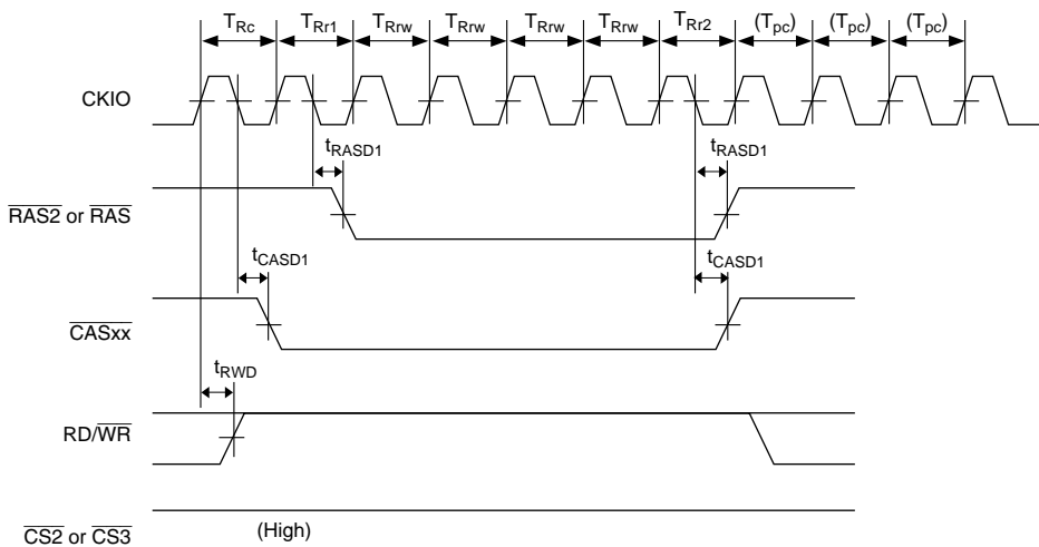
Figure 23.33 DRAM CAS-before-RAS Refresh Cycle (TRAS = 3, TPC = 2)
