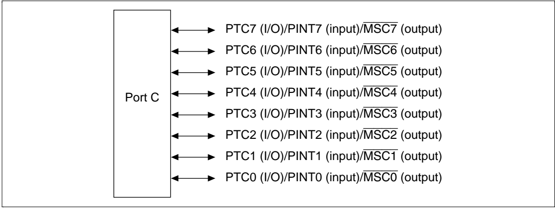
Figure 19.3 Port C
