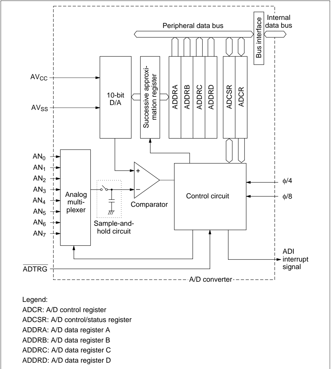
Figure 20.1 A/D Converter Block Diagram
