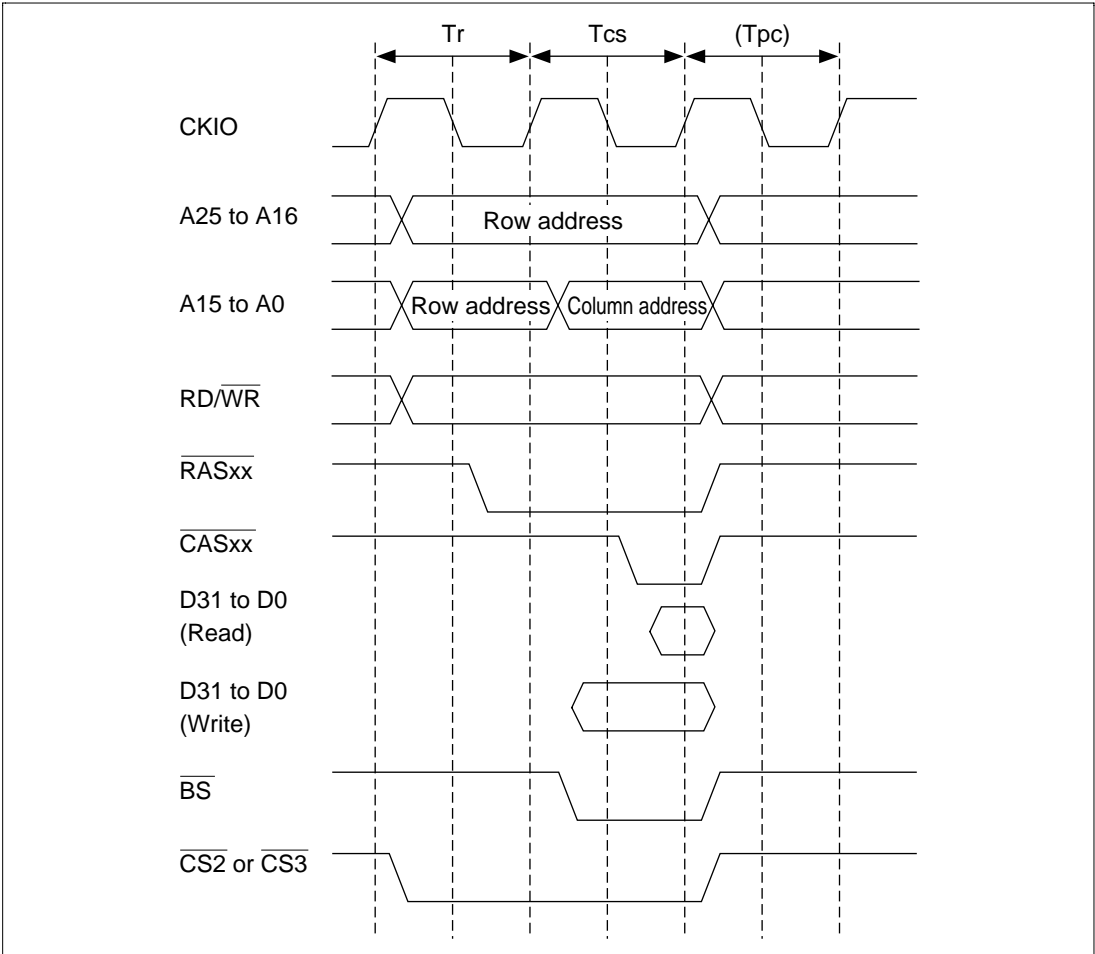
Figure 10.17 DRAM Short-Pitch Access Timing
