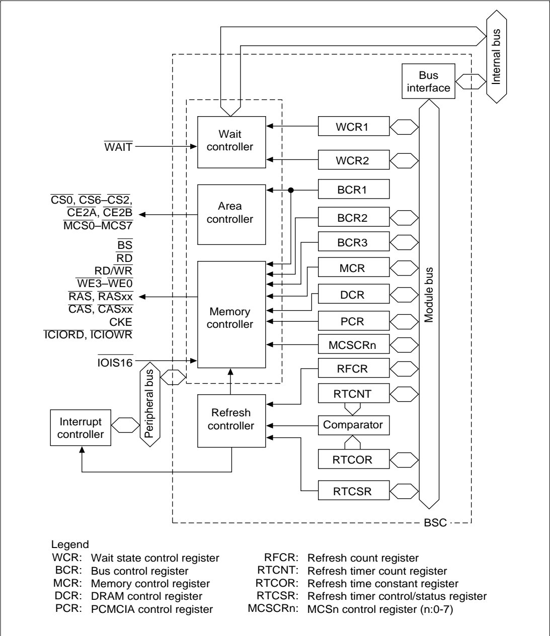
Figure 10.1 BSC Functional Block Diagram
