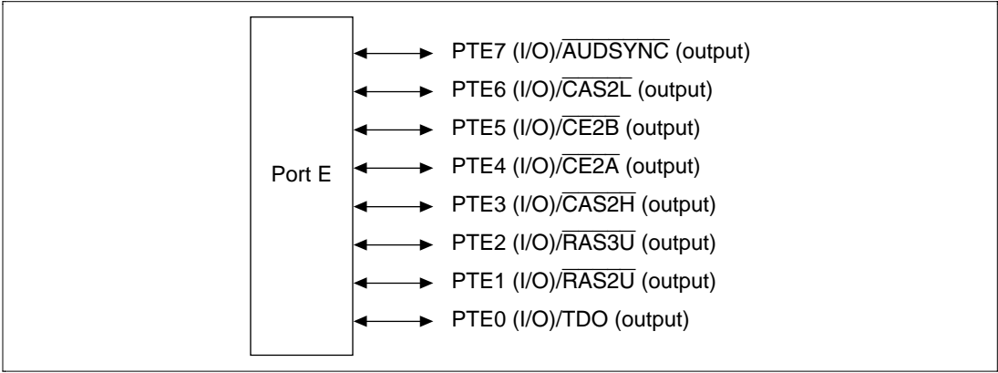
Figure 19.5 Port E
