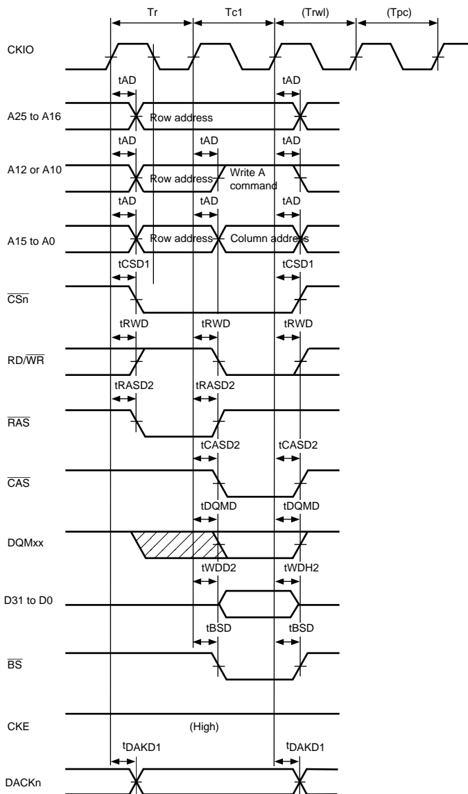
Figure 23.39 Synchronous DRAM Write Bus Cycle ( RCD = 0 , TPC = 0 , TRWL = 0 )
