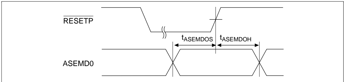
Figure 23.71 ASEMD0 Input Timing
