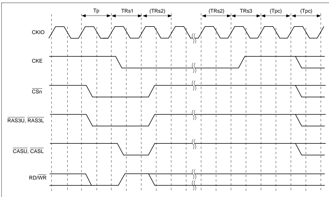
Figure 10.40 Synchronous DRAM Self-Refresh Timing
