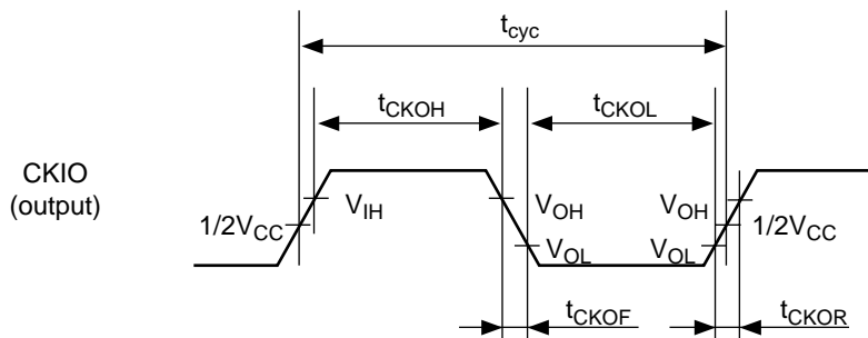
Figure 23.3 CKIO Clock Output Timing
