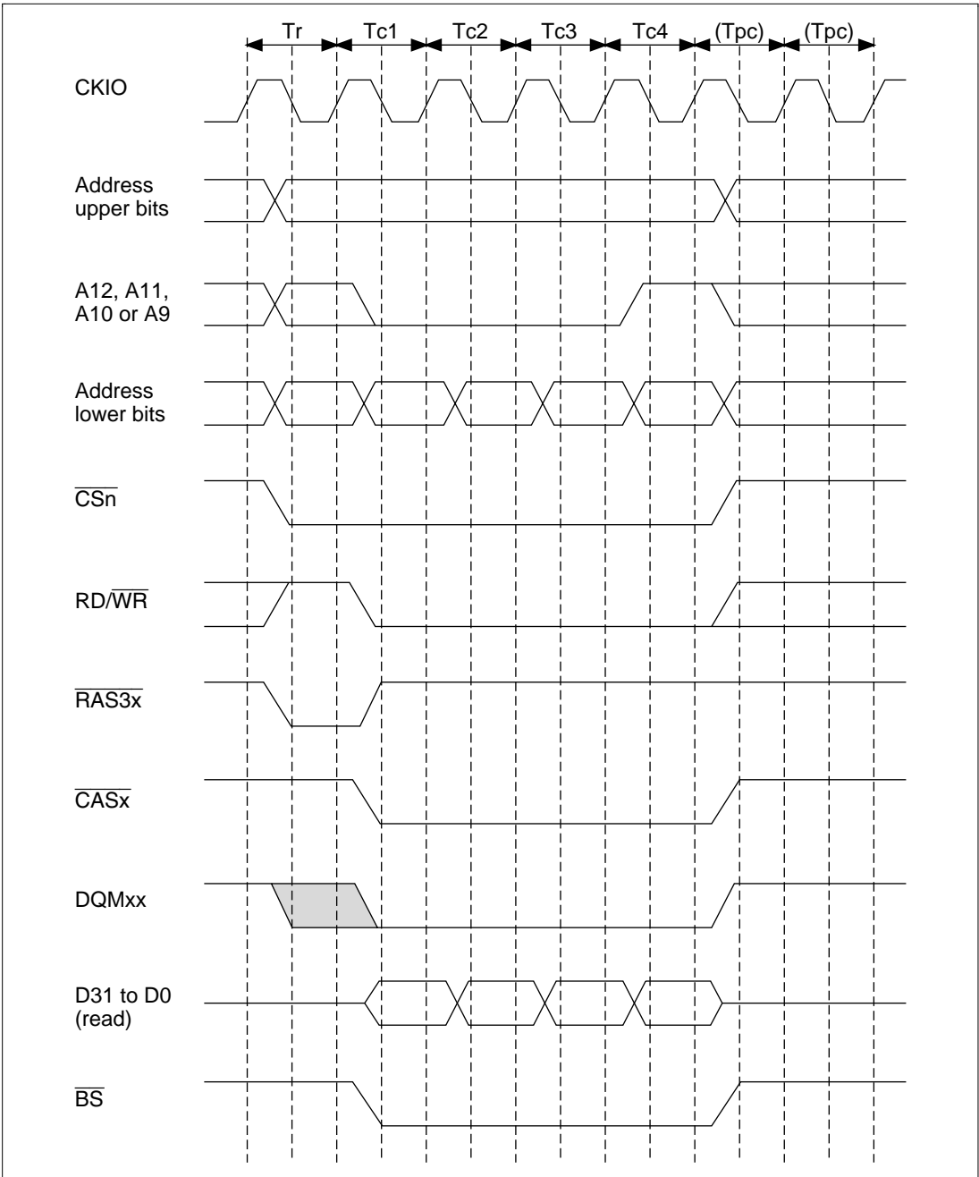
Figure 10.30 Basic Timing for Synchronous DRAM Burst Write
