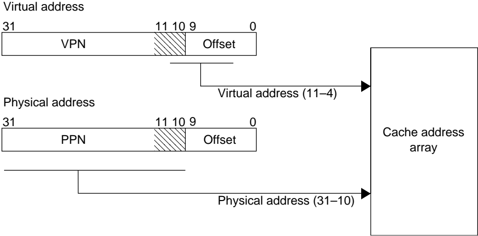
Figure 3.10 Synonym Problem
