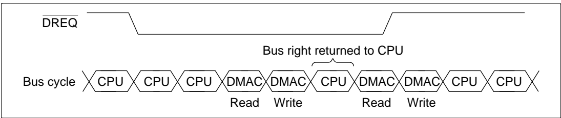
Figure 11.14 Transfer Example in the Cycle-Steal Mode
