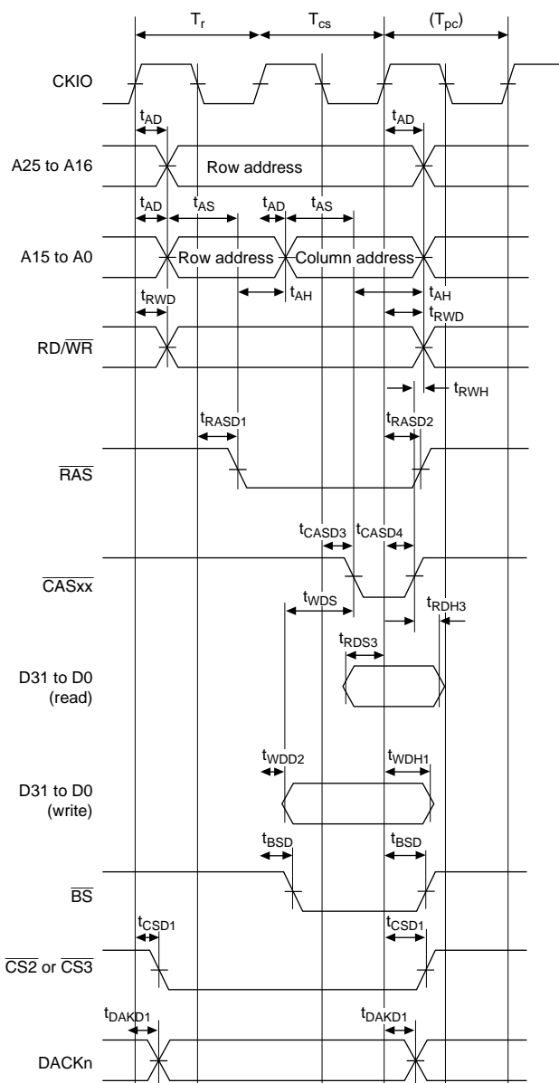
Figure 23.30 DRAM Short-Pitch Access Timing
