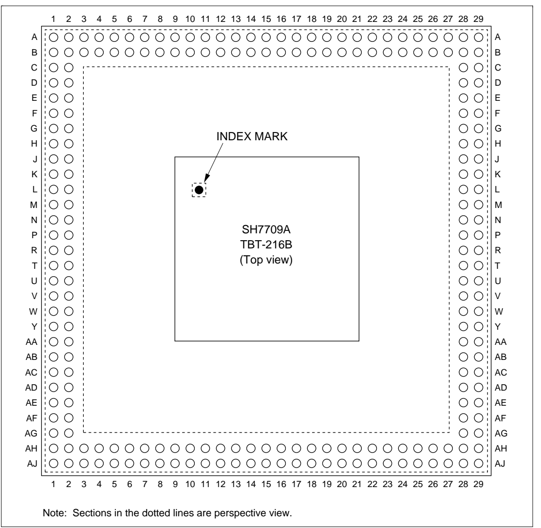
Figure 1.3 Pin Assignment (TBT-216B)
