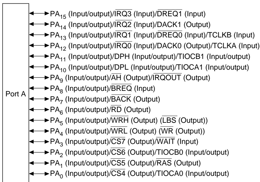
Figure 15.1 Port A Configuration
