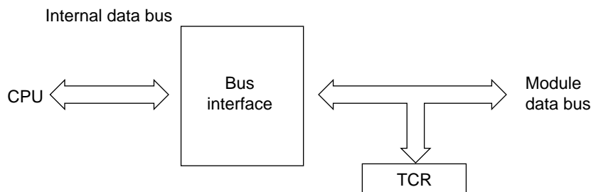
Figure 10.12 TCR Access (CPU-TCR)
