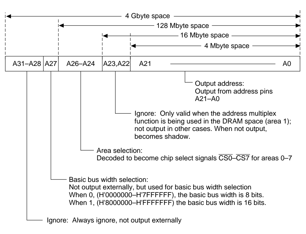
Figure 8.3 Address Format
