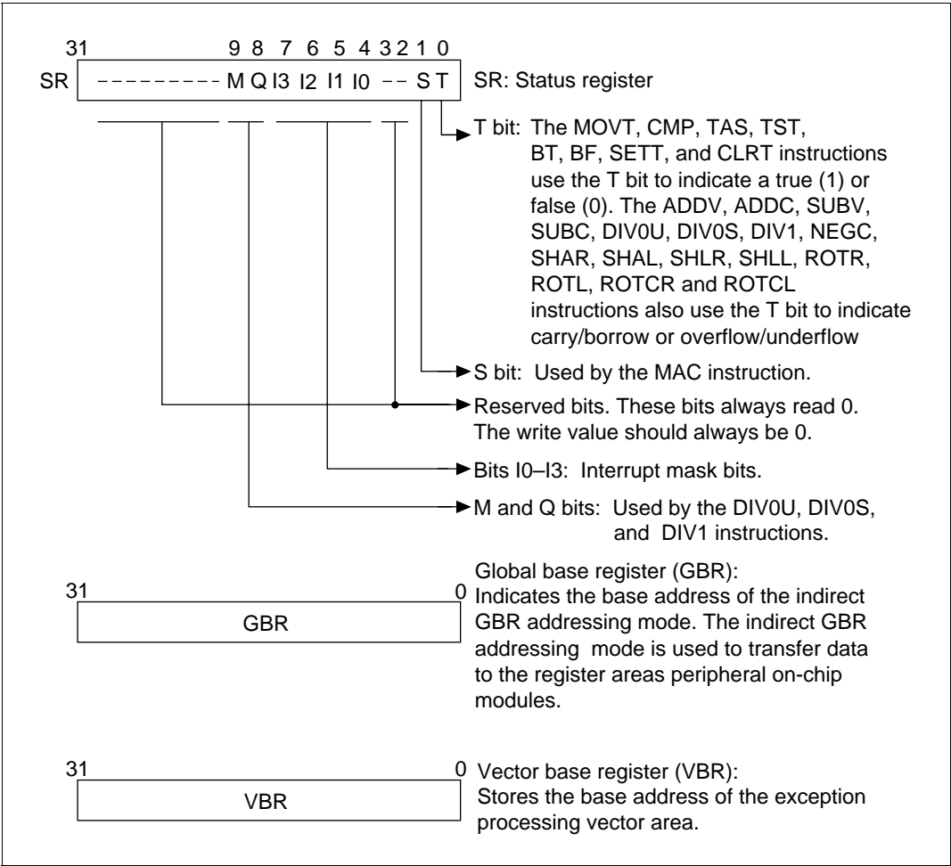
Figure 2.2 Control Registers
