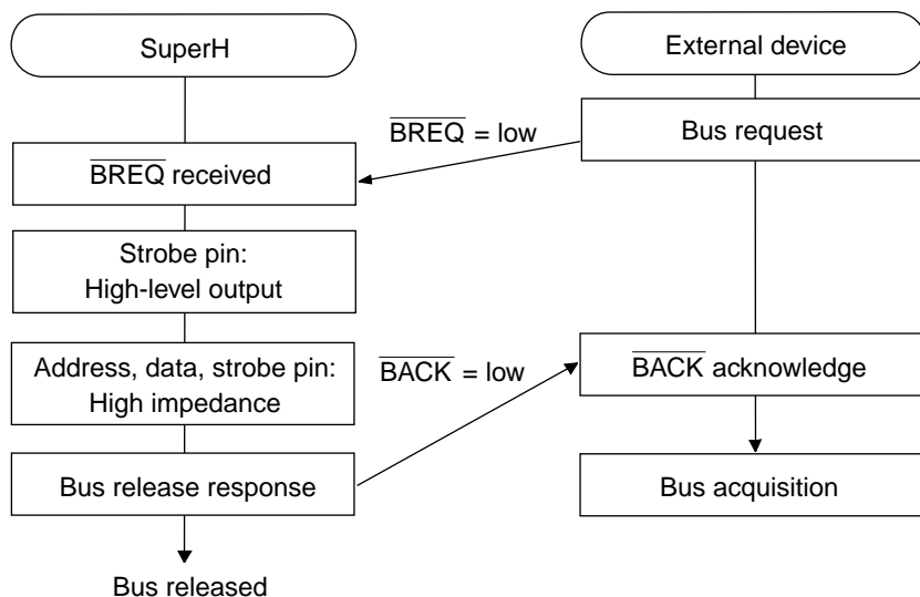
Figure 8.35 Bus Release Procedure
