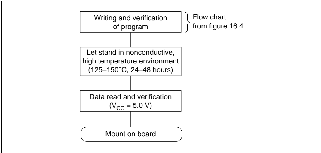
Figure 16.6 Screening Flow
