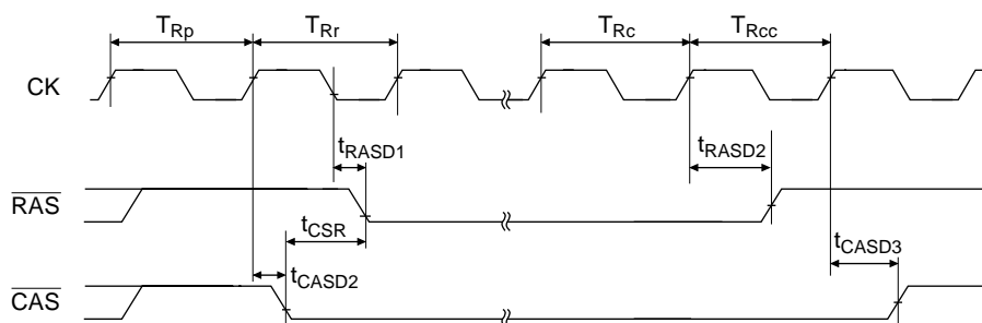
Figure 19.31 Self Refresh
