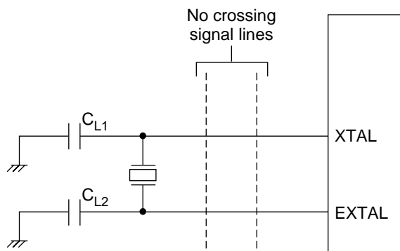
Figure 7.6 Precaution on Oscillator Circuit Board Design
