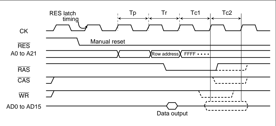
Figure 8.39 Long - pitch Mode Write (2)
