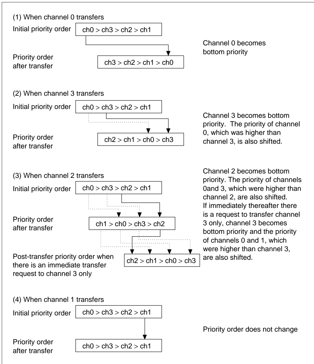
Figure 9.3 Round-Robin Mode
