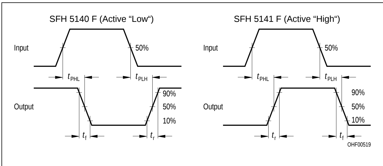
Switching Time Definitions
