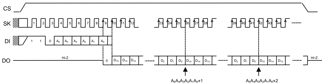
Figure 4 Read Timing (S-29131A)
