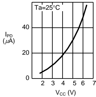
1.11 Pull-Down current I_{PD} - Power supply voltage V_{CC}
